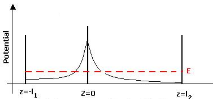
Figure 4: The warping creates a potential barrier for Kaluza-Klein states of the graviton in the Schrödinger coordinate system. States initially localized in the inflationary (left) throat must tunnel through this barrier to communicate with the Standard Model (right) throat. The Schrödinger energy of a state is E = m^2 .
