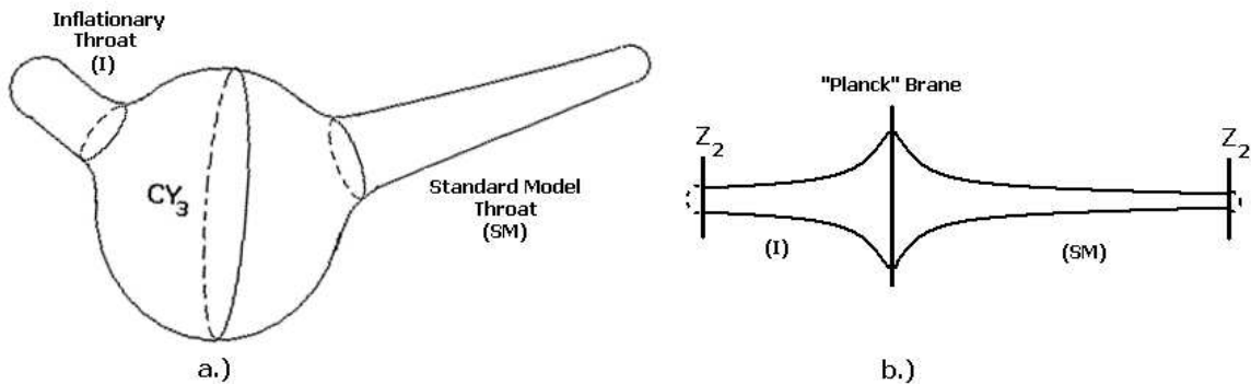
Figure 1: We will consider a KKLMNT setup with two throats, as in (a); as a simplification, we will consider the throats to be AdS_5 , and glue the two throats together at a “Planck” brane, as in (b).
